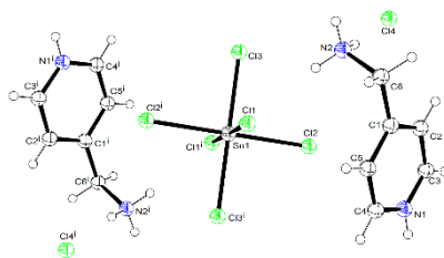
Рис.1. Структура \text{SnCl}_6 \cdot [\text{C}_6\text{N}_2\text{H}_{10}]^{+4} \cdot 2\text{Cl}^{-2}
